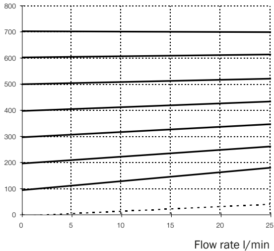
Setting pressure
